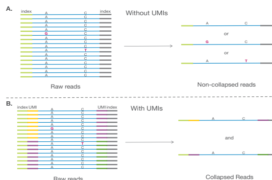
Figure 1: Error correction with DRAGEN™ TruSight Oncology 500 ctDNA Analysis Software —(A) 16 reads with two variants that could be true rare variants or introduced errors. Without error correction, it is impossible to distinguish between true variants and false positives. (B) Integration of UMIs enables recognition of multiple reads from the same starting molecule and collapses them into a single read. Each set of reads contains one error. After error correction, only one correct sequence remains.
