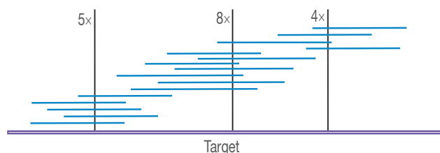
Figure 2: Median exon coverage* —Horizontal lines represent sequencing reads for the targeted region. Vertical lines indicate which reads cover three specific bases. Sequencing depths and positions shown are for illustration only. Every base across a target is considered. The MEC for the region shown is 5x. Recommended MEC for 0.5% LOD following error correction is \geq 1000\times .
